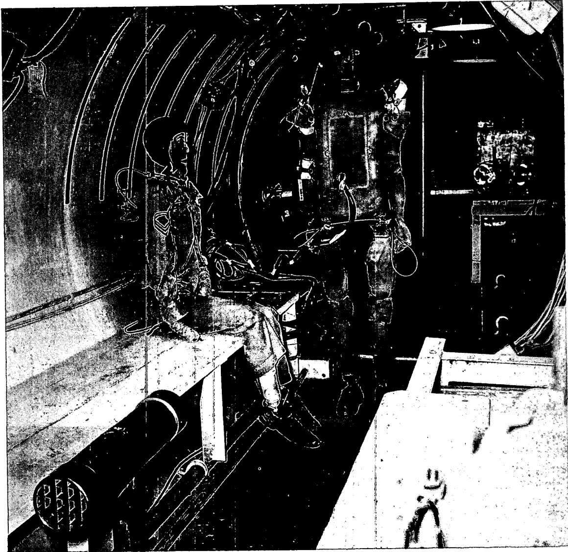
Fig. 3—Dummies in shelter 601. In the left foreground is the drag gauge. The dummy positioning and restraining methods are shown. Accelerometer leads extend from a cavity in the standing dummy.
